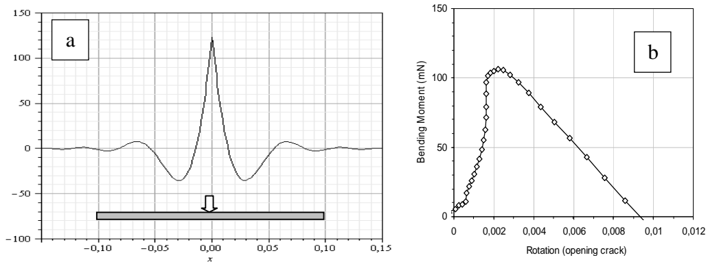
Figure 2. a) Bending moment M(x, T_R) at T_R = 32 \mu s (first fracture time) for a brick specimen b) Bending moment M(0, t) versus rotation \psi(t)
