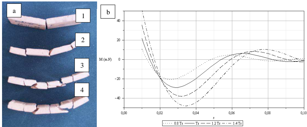
Figure 5. a) Some bricks after the test (strain rate 1: 57 \text{ s}^{-1} , 2: 279 \text{ s}^{-1} , 3: 341 \text{ s}^{-1} , 4: 426 \text{ s}^{-1} ) b) Specimen n°2, bending moment along the beam plotted at several times.
