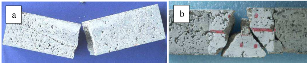
Figure 4. Specimens after the dynamic test. a) Bending failure for a relative loading rate d = 0.38 . b) Shear failure for a relative loading rate d = 7.7 .
