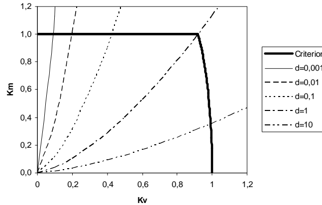
Figure 3. Criterion for a beam made of a quasi brittle material with several loading paths corresponding to several strain rates
