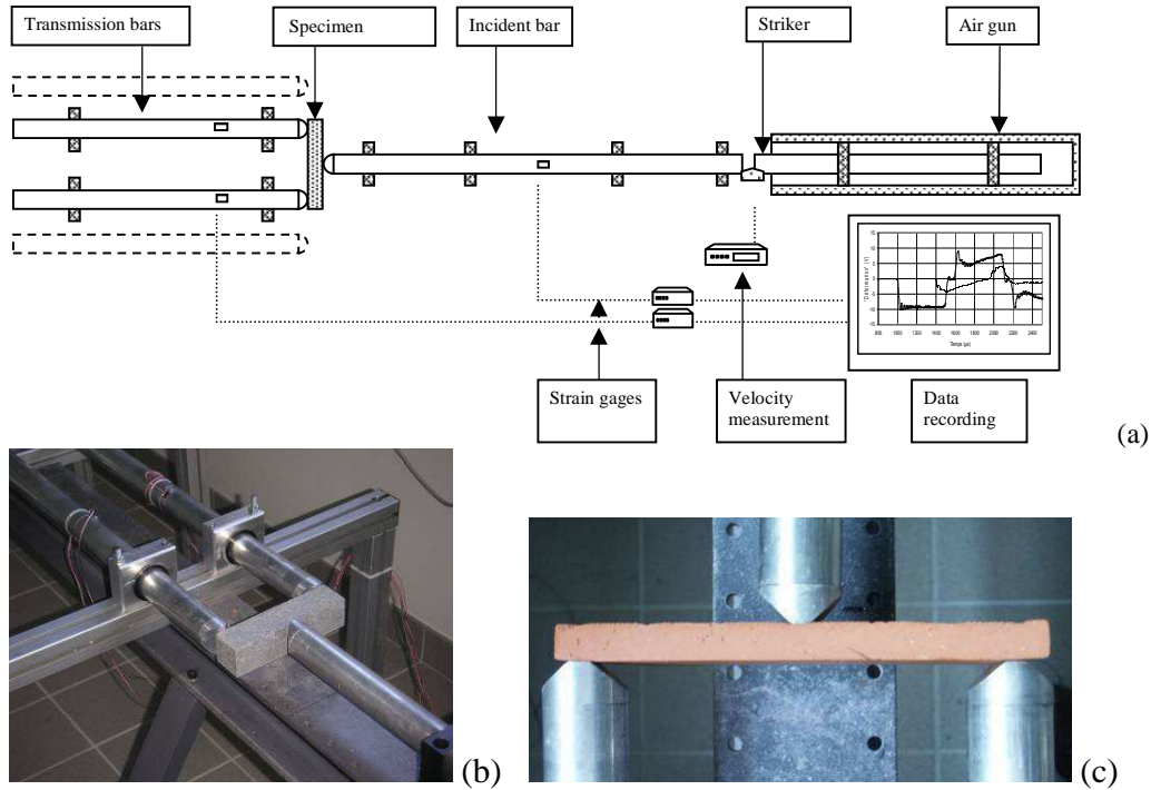
Figure 1. (a) The SHPB device (aluminium bars \phi 40), (b) a micro- concrete specimen, (c) a brick specimen
