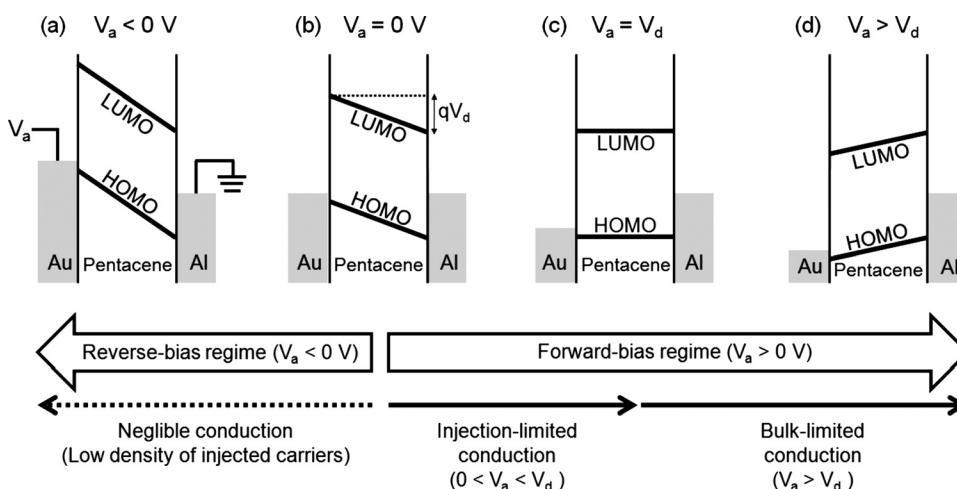
FIG. 3. MIM type energy diagram of a pentacene diode at different operation regimes. (a) Reverse-bias regime, (b) thermal equilibrium, (c) flat-band condition, (d) bulk-limited forward-bias regime. The lower panel indicates the dominant conduction mechanisms under each bias regime.
