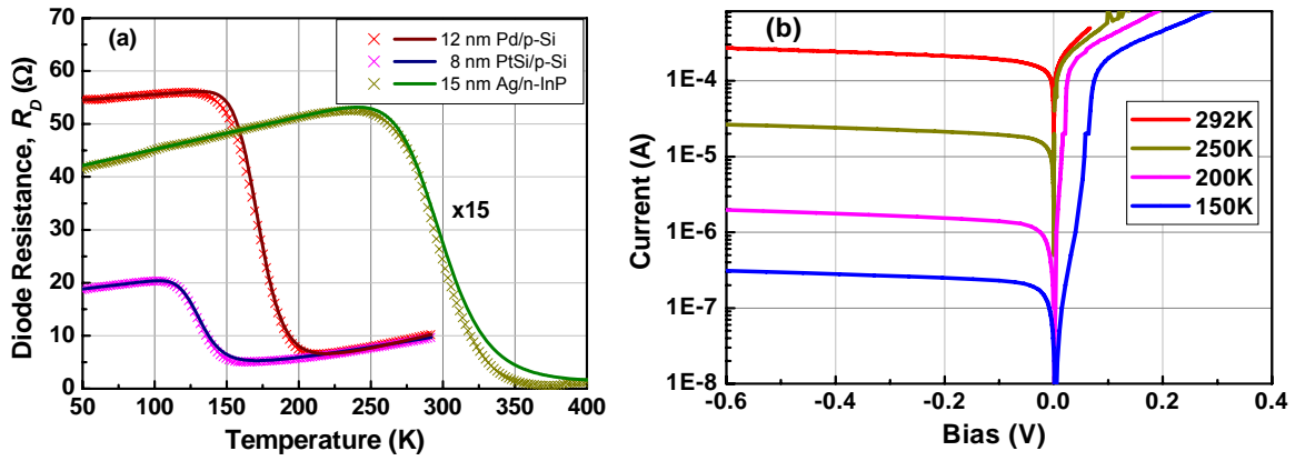
Figure 2. (a) Plots of R_D versus temperature, where the resistance is measured by 4-point probe method with probes contacted to metal electrode of Schottky sample. Symbols are experimental data points and solid lines are modelled curves. (b) Current-Voltage ( I - V ) curves for Pd/p-Si Schottky sample at temperatures indicated on the graph; measurements taken in conventional manner across the Schottky structure via Ohmic back contact and Pd electrode on the front surface of the sample.
