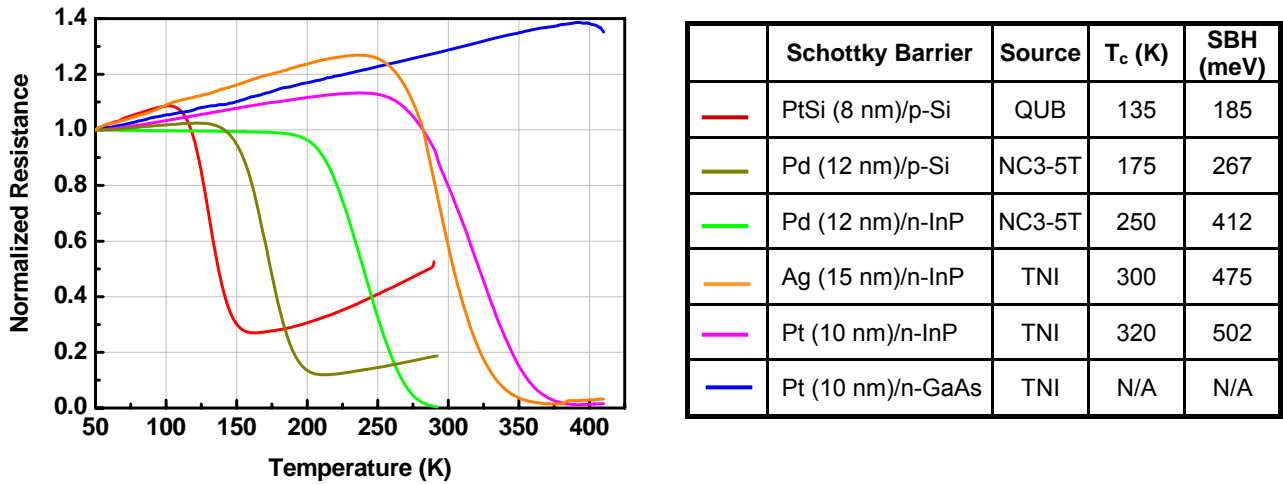
Figure 1. Plots of resistance versus temperature, normalised to resistance at 50 K, where the resistance is measured by 4-point probe method with probes contacted to metal electrode of Schottky sample. Accompanying key and table specifies type of Schottky structure, source of fabrication (QUB – Queen’s University Belfast; NC3-5T – EPSRC National Centre for III-V Technologies, University of Sheffield; TNI - Tyndall National Institute, Cork, Ireland), T_c the mid-temperature of the negative differential resistance (NDR) region and the Schottky barrier height (SBH) at T_c determined from fits of modelled data to the experimental curves (see figure 2).
