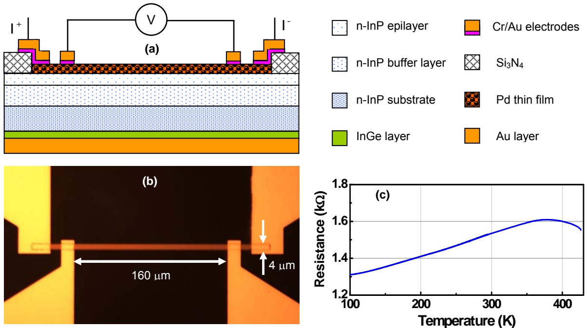
Figure 3. (a) Cross-sectional diagram of Pd/n-InP Schottky diode used for hydrogen detection, drawn in juxtaposition to optical micrograph of actual device, (b). (c) Resistance-temperature plot where resistance is measured by 4-point probe method shown in parts (a) and (b), i.e. probes contacted to only Pd electrode of device which is of width 4 μm and length 160 μm between the two inner voltage probe contacts.
