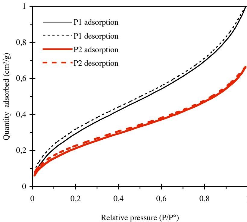
Fig. 1. Argon adsorption and desorption isotherms at 77K, for P1 and P2 samples.
