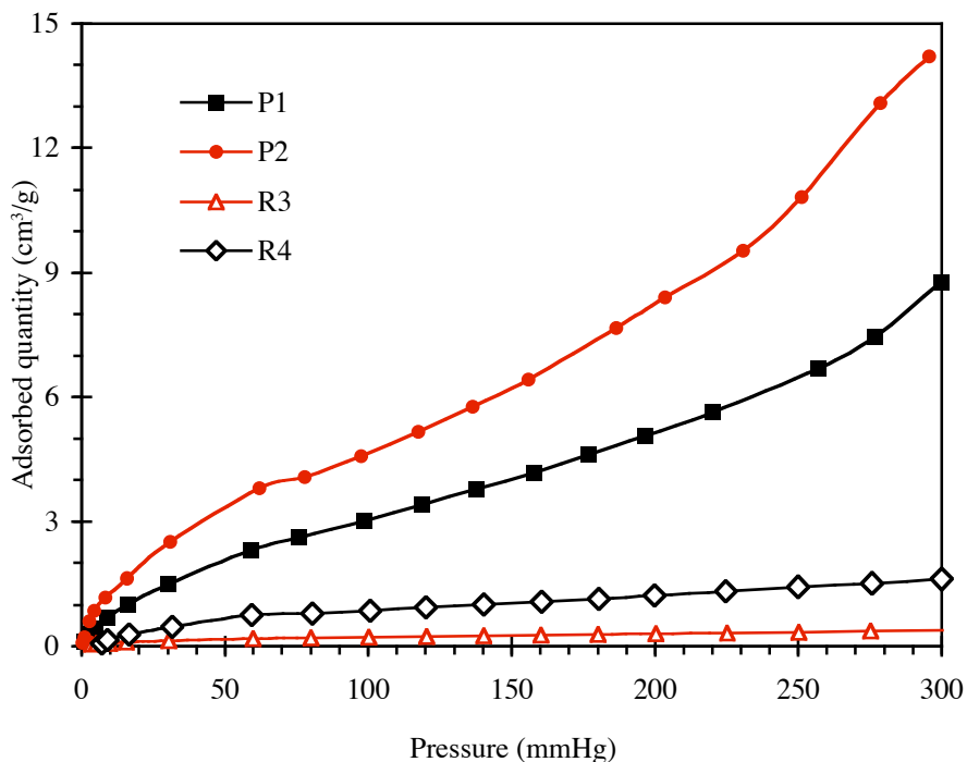
Fig. 3. Butane adsorption isotherms at 273K, for P1 , P2 , R3 and R4 samples.
