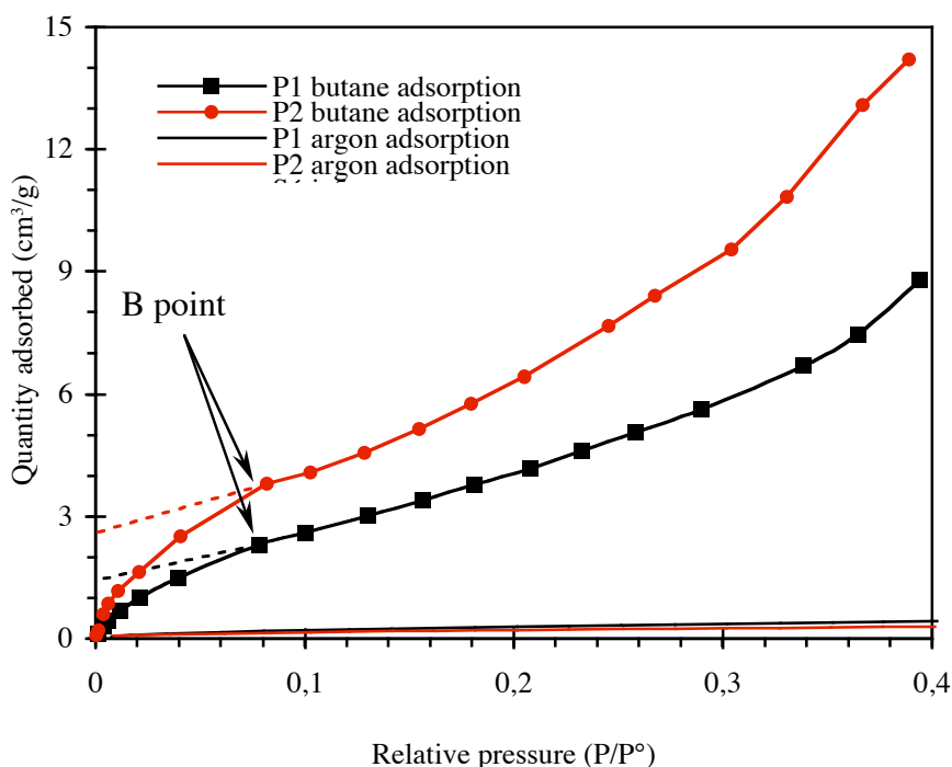
Fig. 2. Comparison between argon adsorption isotherm (obtained at 77K) and butane adsorption isotherm (obtained at 273K), for P1 and P2 samples.
