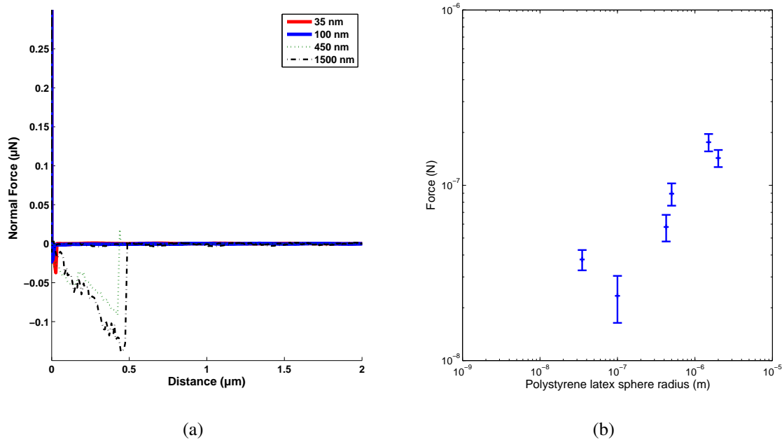
Figure 5: a) Force-distance curves, for a structuring surface by different PS latex particles sizes with a radius of 35 nm (red line), 100 nm (blue line), 450 nm (- - green) and 1.5 \mu\text{m} (- - black); b) the summarize of the measurements. Stiffness: 0.3 N/m and borosilicate radius : 20 \mu\text{m} .
