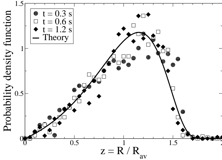
Figure 5. Probability distribution function of the normalized loop sizes for the initial total loops area L^2/4 .
