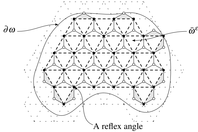
Figure 4. Extending functions to \bar{\omega} . Triangles added in lighter dashed lines. “Small” triangles of \omega_\varepsilon^\varepsilon in gray, see below.
