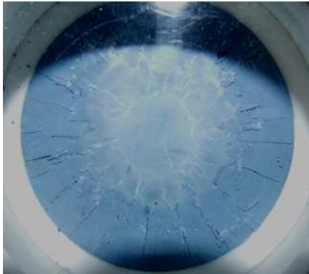
Figure 3: Impact on a target containing inert material I1. Observation of the back face of the sample showing radial and circumferential macro-cracks and a highly compressed zone located at the centre of the face
