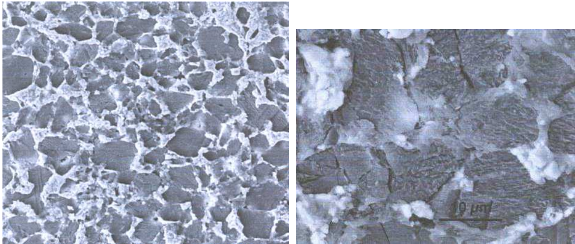
Figure 5: SEM micrographs of material I1 (left, 200 \times 200 \mu\text{m}^2 ). Failure of barium meal in areas where binder is missing and after a biaxial compressive test (right, observed field of 40 \times 30 \mu\text{m}^2 ).
