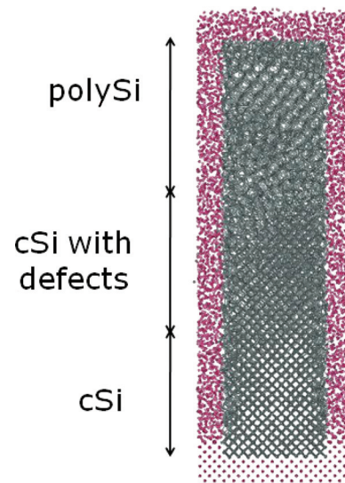
FIG. 10. (Color online) Final structure after 200 ns annealing.
