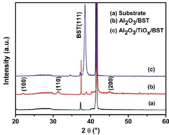
FIG. 8. (Color online) XRD of BST thin films on (001)- \alpha - \text{Al}_2\text{O}_3 substrates buffered with or without a \text{TiO}_x buffer layer (5 nm thick).
