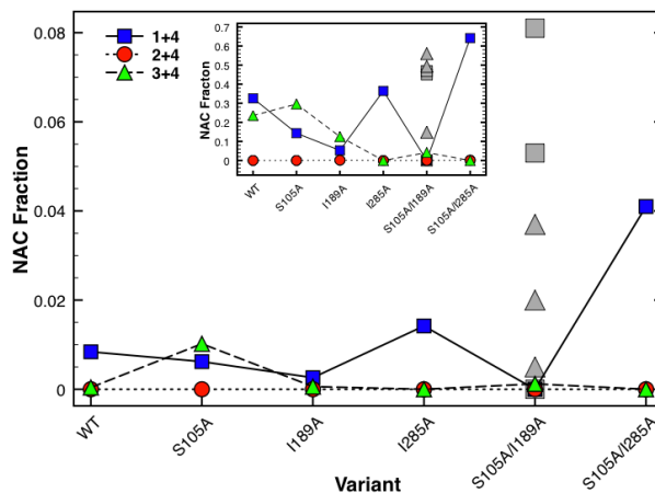
Fig. 6: Simultaneous incipient bond NAC fractions (threshold 4.4 Å). The inset shows corresponding fraction with only one of two distances fulfilled. Results from additional simulations of 1 and 3 in S105A/I189A (see section 3.4) are shown in gray.
