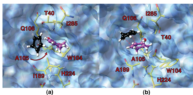
Fig. 9: Selected snapshots from MD simulations of 3 in (a) S105A and (b) S105A/I189A, showing selected residues and hydrogens. In (a) it clearly shows that with both isoleucins present, there is insufficient space above and below the dienophile for TS formation. (b) shows an example of a good NAC conformation. The indicated incipient bond distances are: C_{dne}^{\alpha}-C_{dph}^{\alpha} = 3.79 \text{ \AA} , C_{dne}^1-C_{dph}^{\beta} = 4.15 \text{ \AA} . Closer contact is hindered by T40.
