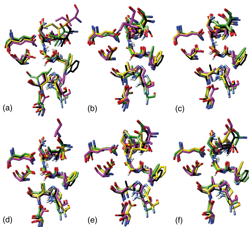
Fig. 2: Superposition of selected residues (40, 104, 105, 106, 134, 157, 187, 189, 224, 285) of the average structure of from simulations in ACN (yellow), CHL (green) and WAT (magenta), relative to the 1LBT crystal structure (black). The superposition was made on the backbone of all 317 residues. For clarity, only selected hydrogens are displayed, belonging to the oxyanion hole or catalytic triad. (a) WT, (b) S105A, (c) I189A, (d) I285A, (e) S105A/I189A, (f) S105A/I285A. Stereoviews of these superpositions are presented in Fig. 6.
