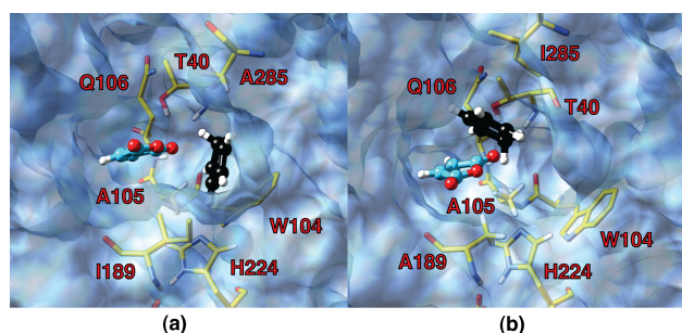
Fig. 8: Selected snapshots from MD simulations of 2 in (a) S105A/I285A and (b) S105A/I189A, showing selected residues and hydrogens. In both illustrations, it is shown how 2 tilts to the left, effectively making the \alpha,\beta -double bond unavailable for attack. (a) shows an unusual diene position, made available because of the dienophile tilt. A more frequent position is shown in (b), but the buriedness of the dienophile hinders attack by the diene.
