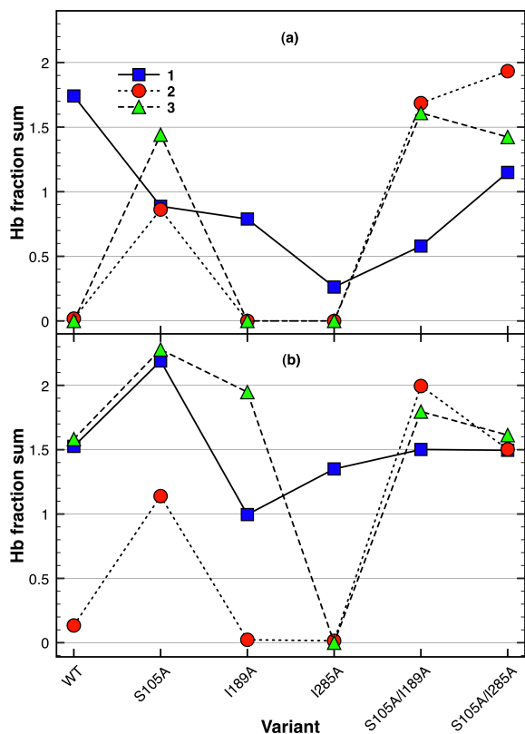
Fig. 5: Sum of fraction of the 3 putative H-bonds between oxyanion hole and substrate acceptor (Q106-NH, T40-NH and T40-O γ H, threshold 2.75 Å), calculated on the last half of each simulation. (a) Dienophile complex, (b) dienophile + diene complex.
