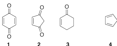
Fig. 3: Structure of Diels-Alder substrates used in this study.
