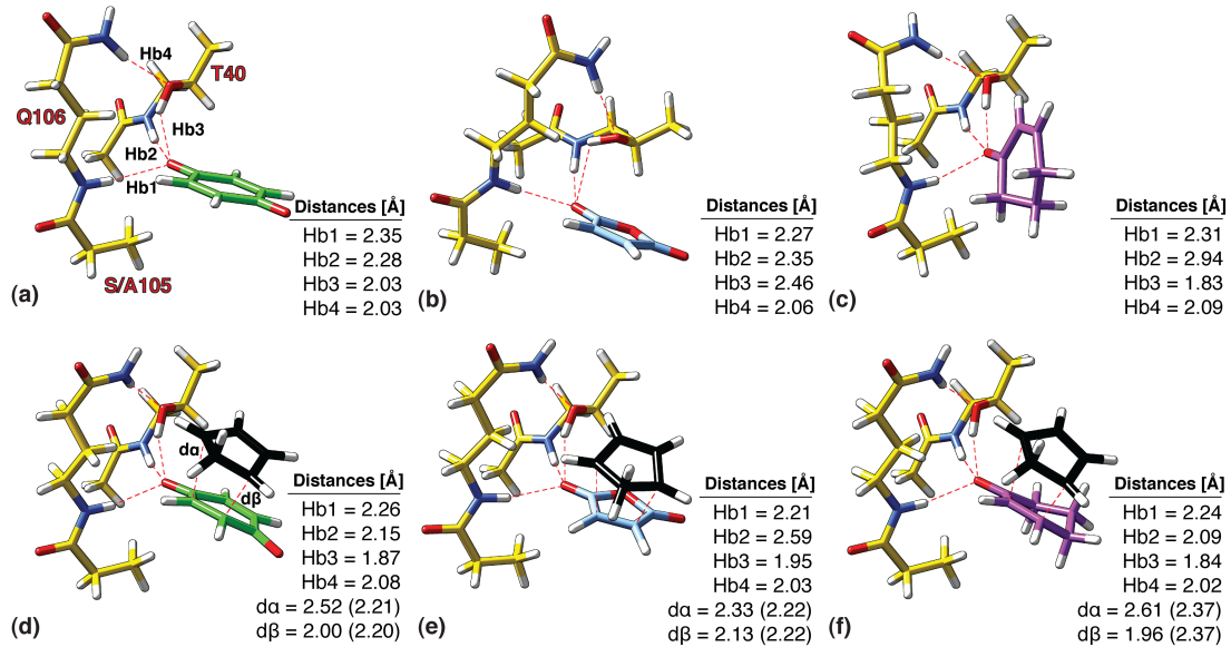
Fig. 11: B3LYP/6-31G(d) optimized geometries of oxyanion hole-bound dienophiles (a-c) and TSs (d-f) model. Distances within parentheses refer to the uncatalyzed TS.
