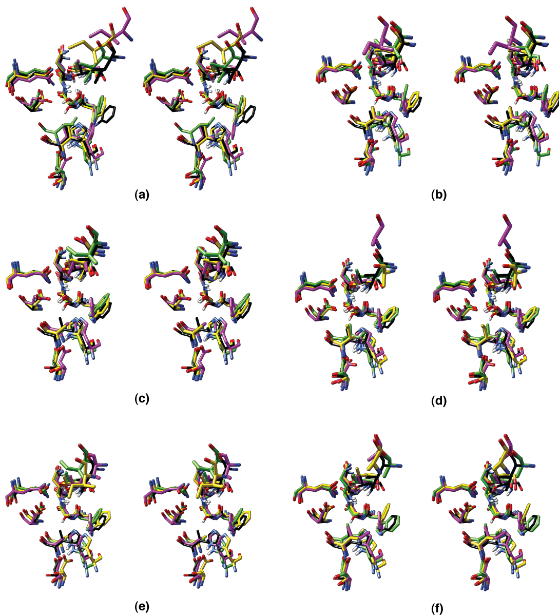
Fig. 6: Stereoviews of selected active site residues of the 6 enzyme variants in the crystal structure 1LBT (black), superimposed with average relaxed structures from ACN (yellow), CHL (green) and WAT (magenta) simulations. For clarity, only selected hydrogens are displayed. (a) WT, (b) S105A, (c) I189A, (d) I285A, (e) S105A/I189A, (f) S105A/I285A.
