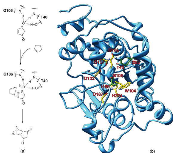
Fig. 1: (a) The hypothetic CALB-catalyzed Diels-Alder mechanism, (b) CALB crystal structure (PDB entry 1LBT), with residues important for the present study explicitly shown. Residues subject to mutations are shown in green.
