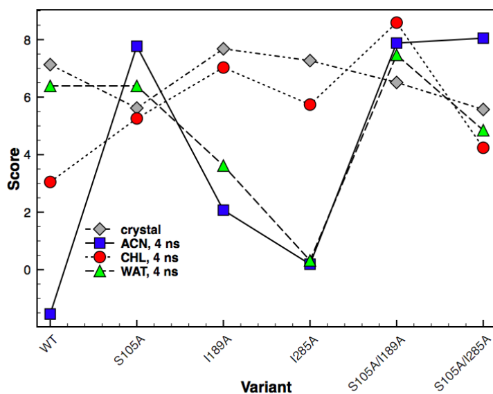
Fig. 3: Sum of composite scores of dienophiles 1-3 in the six enzyme variants, using the crystal structure and solvent-relaxed average structures.
