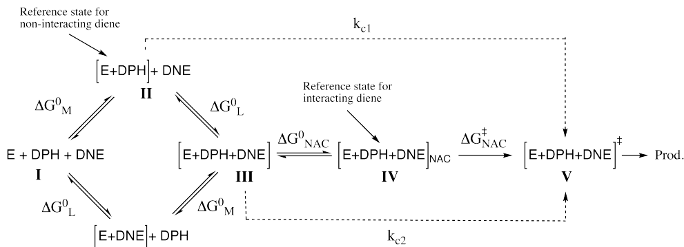
Fig. 2: Reaction pathway showing the difference between the catalyzed and uncatalyzed reactions. \Delta G_M^0 and \Delta G_L^0 refer to the indexing in eqs. 3-11.
