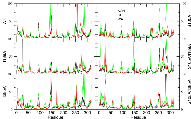
Fig. 1: B-factor per residue, calculated from the 4 ns simulation of the 6 CALB variants, in 3 solvents.
