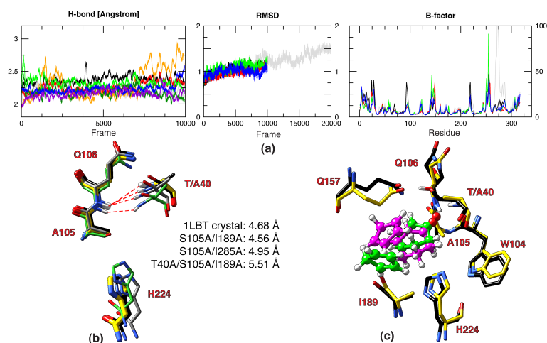
Fig. 4: (a) Simulation statistics of the T40A/S105A/I189A variant. The color legend is as follows: For RMSD and B-factor, gray=naked enzyme; black=dph simulation; red=dph+dne, 1st run; green=dph+dne, 2nd run; blue=dph+dne, 3rd run. For H-bond trajectories (100-frame running averages), Q106 and A40 are represented by black & gray (dph run), red & orange (dph+dne, 1st run), green & dark green (dph+dne, 2nd run), and blue & violet (dph+dne, 3rd run). (b) A comparison of the oxyanion hole geometry between T40A/S105A/I189A (yellow, thick sticks), the 1LBT crystal (green), S105A/I189A (gray) and S105A/I285A (black). All structures refer to the last 200 ps averages of 4 ns relaxation in ACN. His224 is shown for the sake of orientation. The distances displayed are calculated between Q106-N and T/A40-N. (c) Representative snapshots of the [enz·3·4] complexes in T40A/S105A/I189A (yellow, green substrates) and S105A/I189A (black, magenta substrates). Note how the smaller methyl side chain on A40 allows the dienophile to become more buried, and how Q157 moves closer in the triple mutant, both resulting in less accessibility to the \alpha,\beta -double bond. In contrast, the S105A/I189A variant displays a much more ideal NAC-like conformation of the substrates, although the dienophile C ^{\alpha} is still obscured by the T40 side chain.
