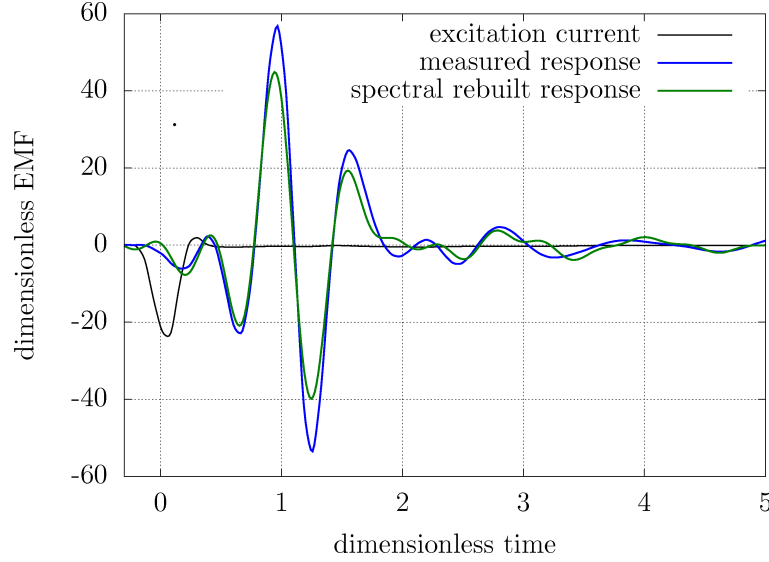
Figure 6: A synthetic response to the pulse in the coil is calculated from the harmonic response and plotted for comparison next to the pulse ( B = 13 T)
