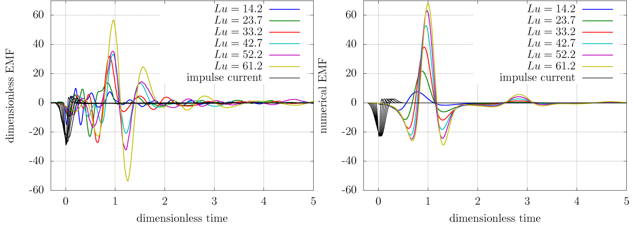
Figure 3: Same as Fig. 2 on the left hand side, except time has been made dimensionless using the propagation time of Alfvén waves and EMF has been made dimensionless using Lu(nI)/(\sigma L) . On the right hand side, the same pulses computed numerically
