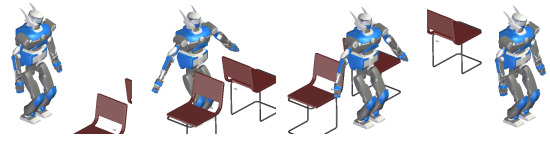
Fig. 2. Collision-free statically stable path for a humanoid robot sliding on the ground.
