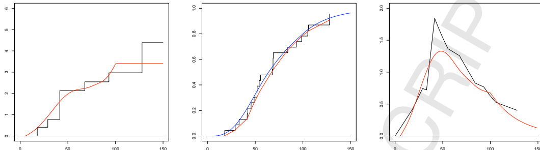
Figure 1: The MLE's and MSLE's based on the ball bearing data on the interval [0, 150] , h = 46 . From left to right: the hazard functions; the empirical distribution function, the estimate corresponding to the MLE (red) and the MSLE (blue); the density estimates.
