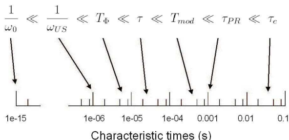
Fig. 2. Order of magnitude of the various times. 1/\omega_0 : optical period; 1/\omega_{US} : acoustic period; T_\phi : acousto-optical correlation time; \tau : time averaging characteristic time; T_{mod} : characteristic time of the modulation H(t) ; \tau_{PR} : photorefractive time; \tau_c : Lock-in integration time.
