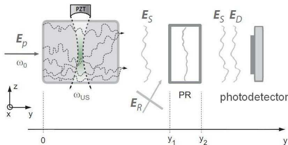
Fig. 4. Principle of the photorefractive detection.
