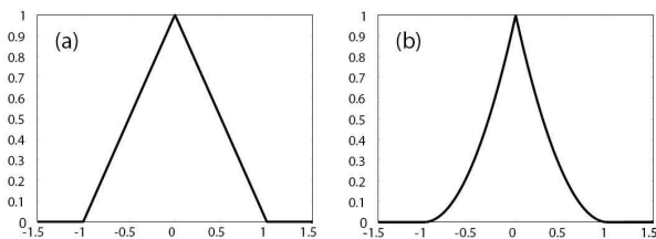
Fig. 3. Plot of correlation function g_1(\theta) (a), and its square |g_1(\theta)|^2 (b). The horizontal axis Units is either \theta/T_\Phi (for time correlation), or (z - z_0)/\Delta z with \Delta z = c_{US} T_\Phi (for z resolution).
