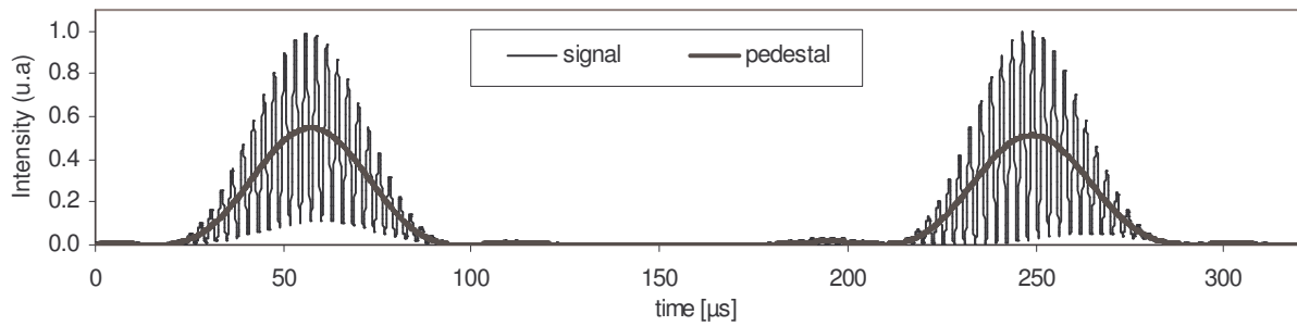
Fig. 7. Typical signal of GS-PDA
