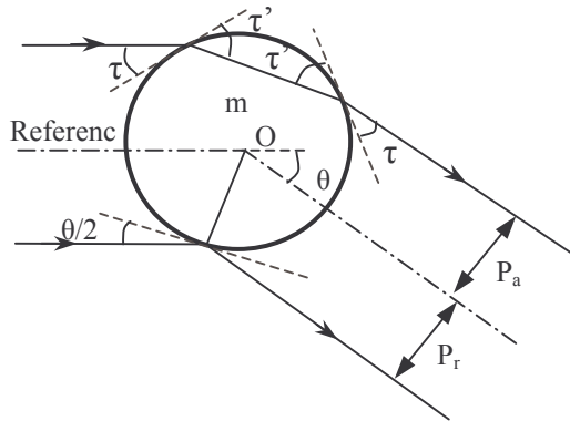
Fig. 3 Optical paths
