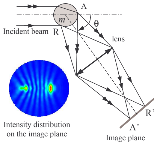
Fig. 1. Off-axis imaging and intensity distribution on the image plane
