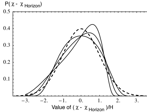
Figure 2. Expected one-point probability distribution of the isocurvature perturbation in case of a quartic potential (solid lines). The plot corresponds to the case \nu^2(N_c - N_*)/9 = 1 . Finite volume effects can shift the Hubble size value of \chi to a non-zero value \chi_{\text{Horizon}} for our observable universe leading to a skewed distribution of \chi . The three solid lines correspond to \chi_{\text{Horizon}}/H = 1, 0.5 and 0 . The dashed line is a Gaussian distribution of the same width. See Ref. [36] for details.
