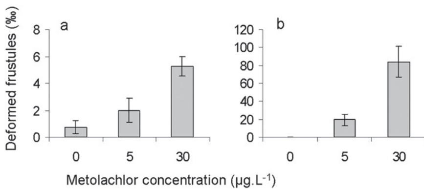
Fig. 7. Relative abundance of deformed frustules (± S.E.) in the whole diatom community (a) and within Surirella angusta populations (b). Kruskal–Wallis test: p < 0.05 (a) and p < 0.01 (b).
