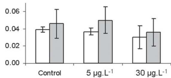
Fig. 2. Biofilm biomass ( \pm s.e.) on glass slides after 14 days of experiment, expressed as ash-free dry mass (AFDM, white bars, \text{mg.cm}^{-2} ) and as chlorophyll-a (grey bars, \text{mg.dm}^{-2} ).
