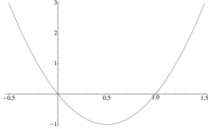
Figure 6.3: The entropic functional e_{p,+}(\alpha) of the open XY-chain.
