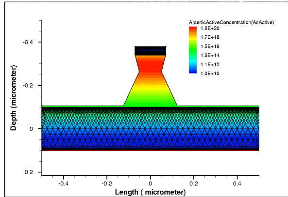
Fig. 6. The simulated counterpart for a 130 nm configuration. The arsenic gradient in the silicon layer is shown.
