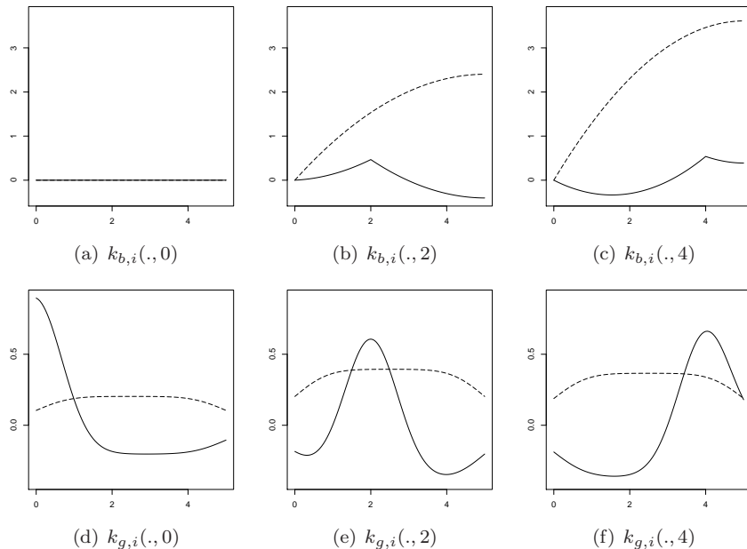
Figure 2: Representation of the kernels k_{b,i}(\cdot, y) and k_{g,i}(\cdot, y) for y = 0, 2, 4 and i = 0, 1 . The dashed lines correspond to k_{b,1}, k_{g,1} and the solid lines are for k_{b,0} and k_{g,0} . The original kernels k_b(\cdot, y) and k_g(\cdot, y) can be retrieved by summing the two curves.
