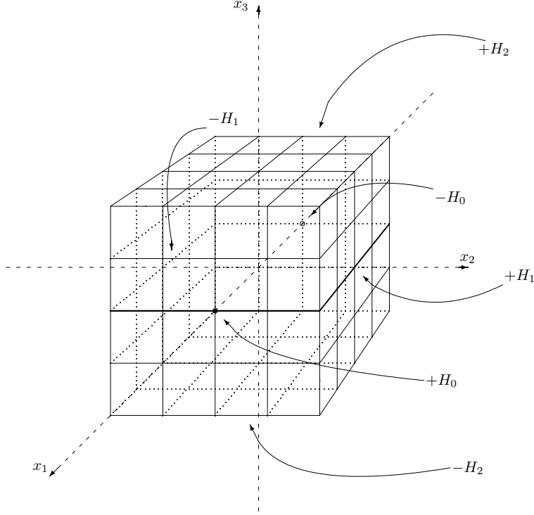
FIGURE 1. An illustration of \mathbf{M} for n = 2 and t = 2 .
