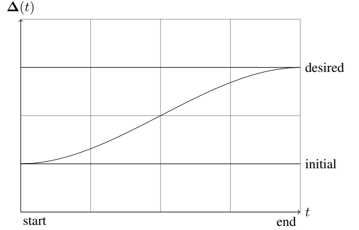
Fig. 5. Polynomial curve \Delta(t) providing a smooth transition between feet and center of mass trajectories.
