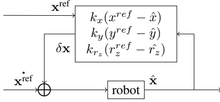
Fig. 3. Naive correction system for a humanoid robot. \mathbf{x}^{\text{ref}} = (x^{\text{ref}}, y^{\text{ref}}, r_z^{\text{ref}}) , \dot{\mathbf{x}}^{\text{ref}} = (\dot{x}^{\text{ref}}, \dot{y}^{\text{ref}}, \dot{r}_z^{\text{ref}}) and \hat{\mathbf{x}} = (\hat{x}, \hat{y}, \hat{r}_z) are respectively the current planned robot position, velocity and position estimated by an external localization system. The planned control \dot{\mathbf{x}} is rectified by summing \delta\mathbf{x} a correction directly computed by the position error of the waist between the plan and the perception.
