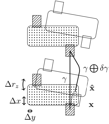
Fig. 4. Correction of the next step due to a position error. Dotted rectangles are the planned positions \mathbf{x} of the robot waist and feet before and after the next step. Non-dotted rectangles corresponds to the robot localization \hat{\mathbf{x}} . Error w.r.t to axis X, Y and yaw rotation is (\Delta x, \Delta y, \Delta r_z) = \delta\mathbf{x} , \gamma the reference trajectory and \delta\gamma the corrected trajectory reaching the planned step.
