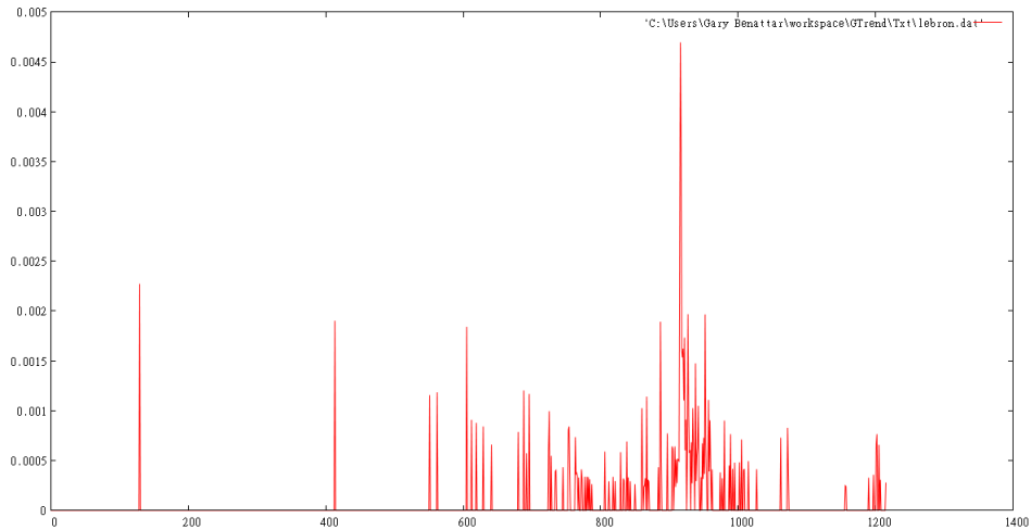
Figure 16: p('lebron')
