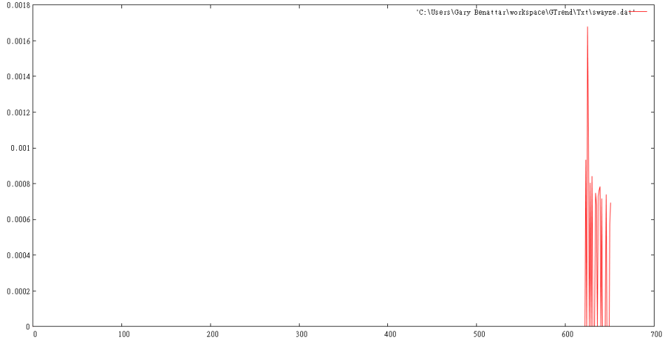
Figure 15: p('swayze')
