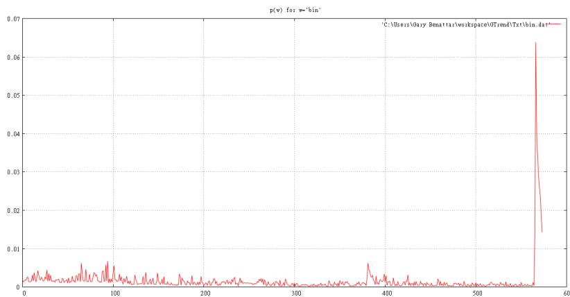
Figure 1: p('bin')
