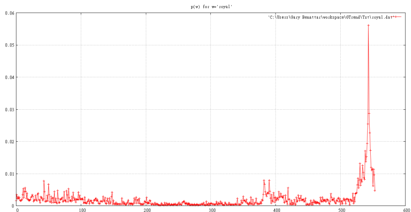
Figure 2: p('royal')
