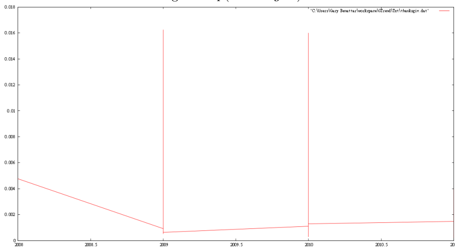
Figure 9: p('thanksgiv')
