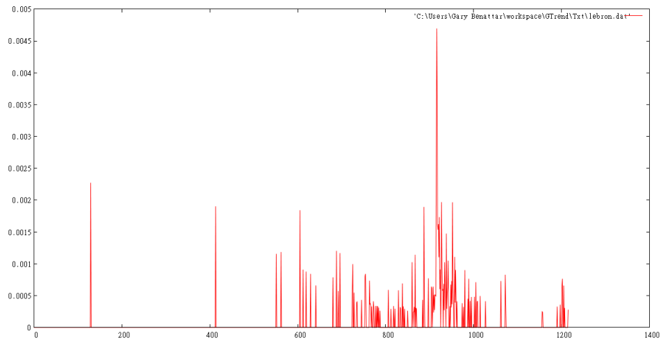
Figure 16: p('lebron')
