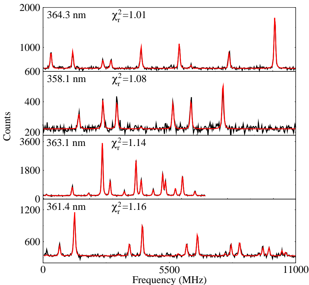
Figure 2. Hyperfine structures of the 364.3 nm, 358.1 nm, 363.1 nm and 361.4 nm lines for the stable ^{45}\text{Sc} isotope investigated during the off-line preparation tests. Fitted Voigt profiles are also shown.
