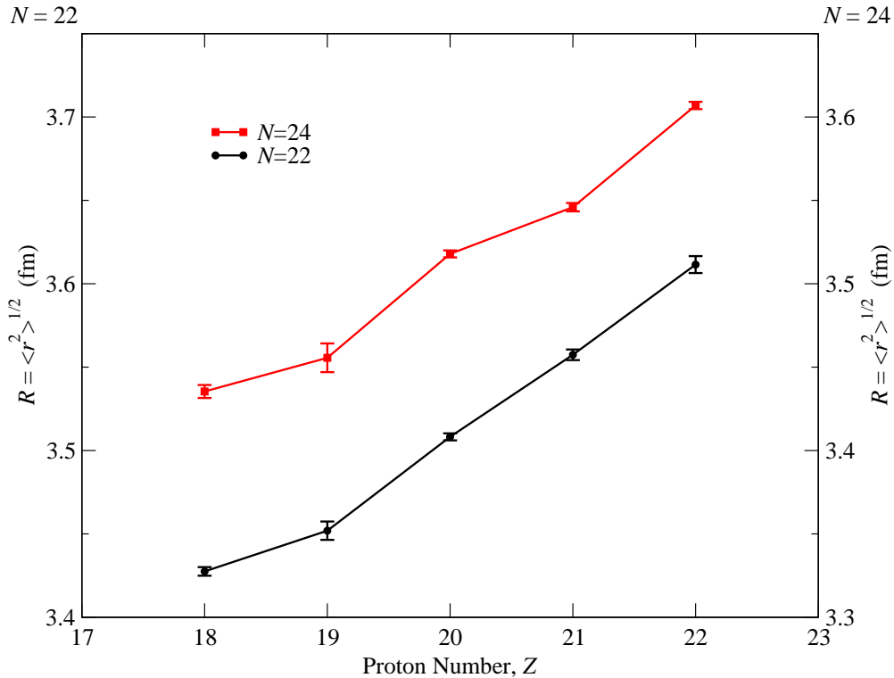
Figure 6. Isotonic dependence of rms nuclear charge radii in the f_{7/2} shell.
