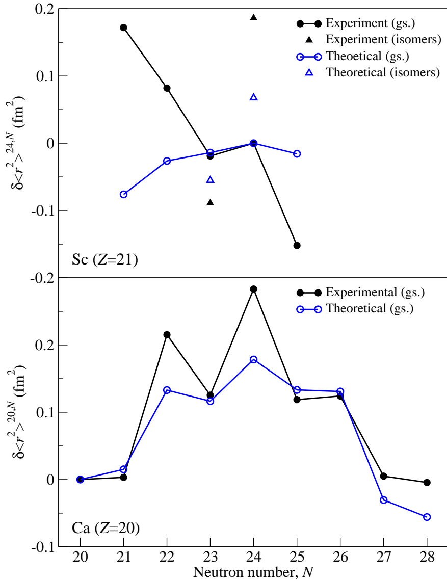
Figure 7. Comparison of experimental Ca and Sc ms charge radii with theoretical estimates performed as part of this work.
