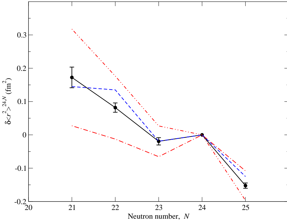
Figure 4. Neutron number dependence of the ^{42-46}\text{Sc} charge radii. Experimental data are denoted by full circles and the error bars represent statistical errors; the two enveloping lines indicate the effect of the specific mass shift uncertainties of 25%. The dashed line represents a fit to the Zamick formula [39].
