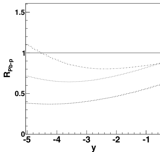
Figure 2. J/\psi 's R_{Pb+p} ratio versus rapidity for different values of transverse momentum: 2.5 GeV/ c (dashed line), 5 GeV/ c (dotted line) and 10 GeV/ c (dash-dotted line). These results are obtained from numerical CGC simulations only and were calculated at \sqrt{s} = 8.8 TeV.
