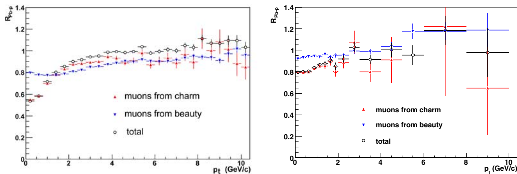
Figure 1. The nuclear modification factor R_{Pb-p} is presented for both CGC and MNR+EKS98 calculations on the left and right hand side, respectively. These results are obtained at the generation level only. See text for more details.
