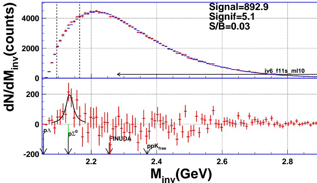
Figure 4. Reconstructed invariant mass of \Lambda - proton pairs. The solid histogram and crosses denote the data (red) and the scaled mixed-events background (blue), respectively (upper panel). Both distributions were normalized over the range indicated by the horizontal arrow. The lower panel shows the difference and an excess at a mean value M(p\Lambda) = 2.134 \pm 0.004 GeV with a width of \Gamma = 26 \pm 14 MeV (statistical errors only). The statistical information (signal strength, significance and signal-over-background ratio) is extracted in the mass range limited by the vertical dashed lines shown in the upper panel.
