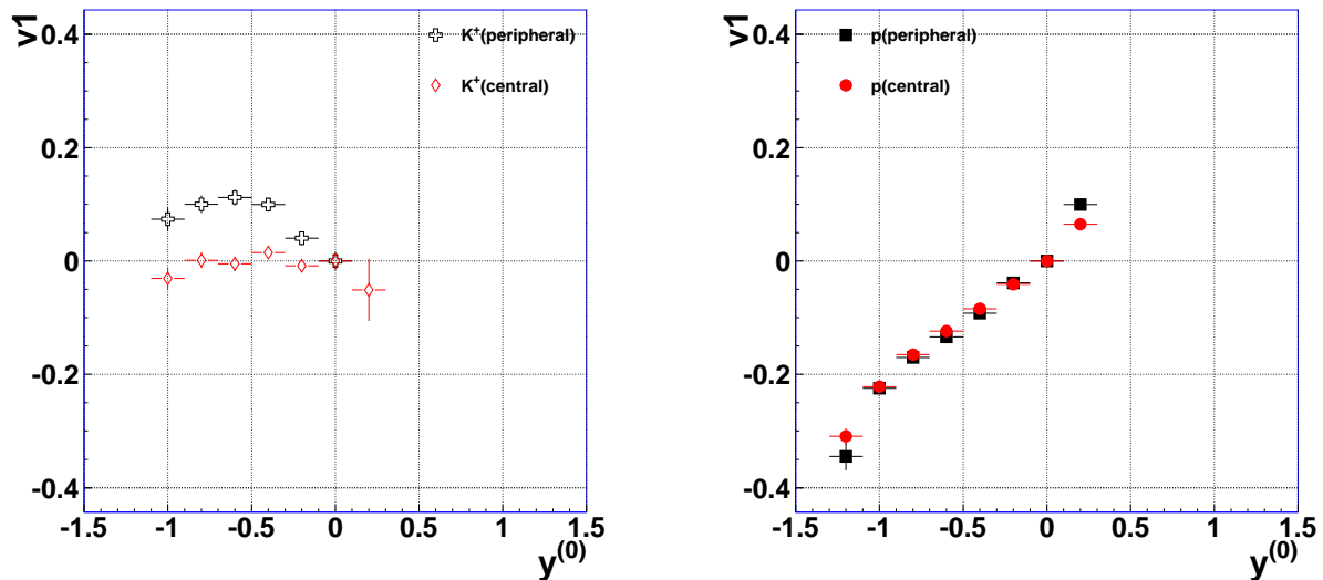
Figure 2. Sideflow of kaons and protons in the reaction Ni+Ni at an incident energy of 1.91 AGeV as function of normalized rapidity y^{(0)} = y/y_{CM} - 1 . The first Fourier coefficients v_1 are plotted for two different centrality bins for kaons (left panel) and protons (right panel). Black data points are obtained for peripheral collisions corresponding to a mean impact parameter of 6 \pm 1 fm, the red ones for central collisions with a geometrical impact parameter b < 3 fm. The v_1 -values are obtained within the acceptance of the CDC, for details see text.
