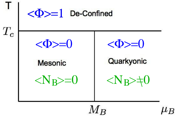
Figure 1. The phase diagram in large N_c proposed in [2].
