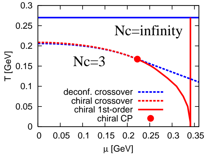
Figure 2. The phase diagram of a PNJL model for different N_c [3]. Two straight lines indicate the deconfinement and chiral phase transitions for N_c = \infty and the lower curves for N_c = 3 .
