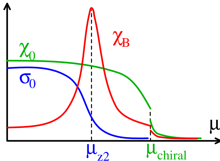
Figure 5. The behavior of the baryon number susceptibility as a function of chemical potential.
