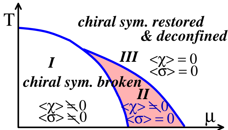
Figure 4. Schematic phase diagram mapped onto (T, \mu) plane. The lines do not distinguish the order of phase transitions. The critical point can appear on the boundary that separates the phase I from III at low \mu and/or the phase I from II at intermediate \mu [15].
