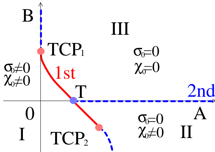
Figure 3. Phase diagram with C = -1 , D = F = 0 and h = 0 [15]. The solid and dashed lines indicate first and second order phase boundaries, respectively. One tricritical point, TCP_1 , is located at (A, B) = (0, 1/4) and another, TCP_2 , at (A, B) = (1/4, -1/8) . The triple point represented by T is at (A, B) = (1/8, 0) .
