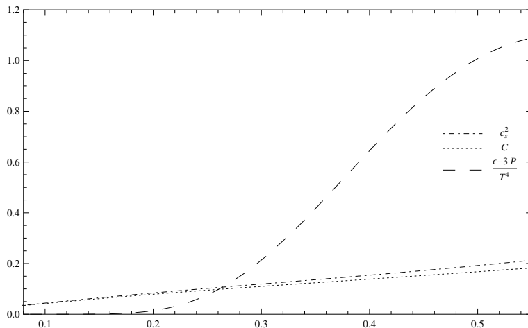
Figure 7. The NP velocity of sound, conformity and the trace anomaly relation as functions of T/T_c . They are shown in the low-temperatures region up to 0.6T_c .
