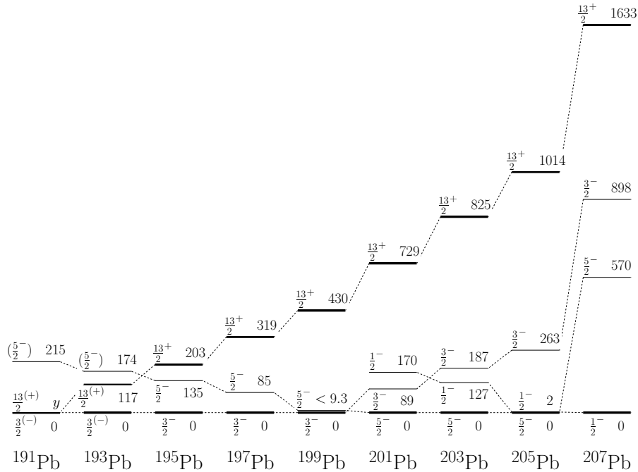
Figure 9. Systematics of the lowest-lying energy levels with spin and parity \frac{1}{2}^{-} , \frac{3}{2}^{-} , \frac{5}{2}^{-} , and \frac{13}{2}^{+} in neutron-deficient odd- A Pb isotopes. These levels are dominated by one-quasiparticle excitations of the \nu 3p_{1/2} , \nu 3p_{3/2} , \nu 2f_{5/2} , and \nu 1i_{13/2} orbitals, respectively. This extends the previous systematics presented in Ref. [21]. Note that the order of the lowest energy states ( \frac{3}{2}^{-} , \frac{13}{2}^{+} ) in ^{191}\text{Pb} and their relative excitation energy y are not known.
