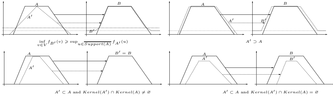
Fig. 3. Some properties of GMP conclusions given Lukasiewicz's implication
