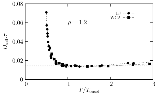
FIG. 9: Decoupling between the T dependences of the self diffusion constant D_{\text{self}} and of the relaxation time \tau for \rho = 1.2 as a function of the temperature T rescaled by the independently measured T_{\text{onset}} . For both models, the product D_{\text{self}} \tau begins to increase below T \approx T_{\text{onset}} , which differ by a factor 1.6 for both models, see Table I.
