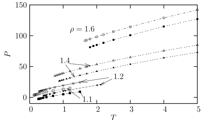
FIG. 1: The P(T) equation of state for the LJ (filled symbols) and WCA (open symbols) models at different densities merely differ by a constant.
