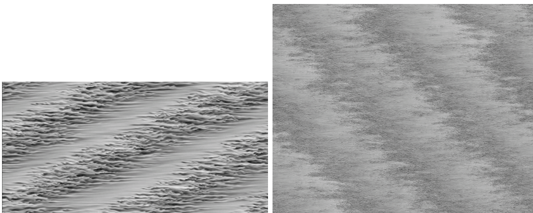
Figure 1: Streamwise velocity in the mid-plane between the plates. The mean flow direction is horizontal. Left: non-rotating pCf for Re=350 . Right: rotating pCf for Re=6000 and Ro=-0.104 . Domain sizes: 250h \times 125h (top) and 250h \times 200h (bottom).
