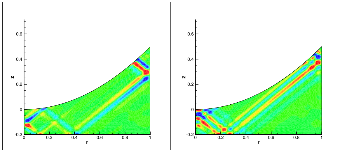
Figure 1: Exemples of singular eigenmodes in a tank with a parabolic surface
