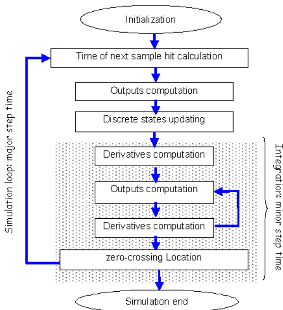
Fig. 2. The principle of variable step simulation in Simulink
