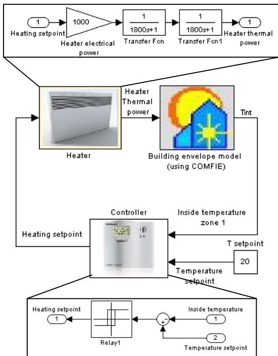
Fig. 5. Complete coupling schema in Simulink
