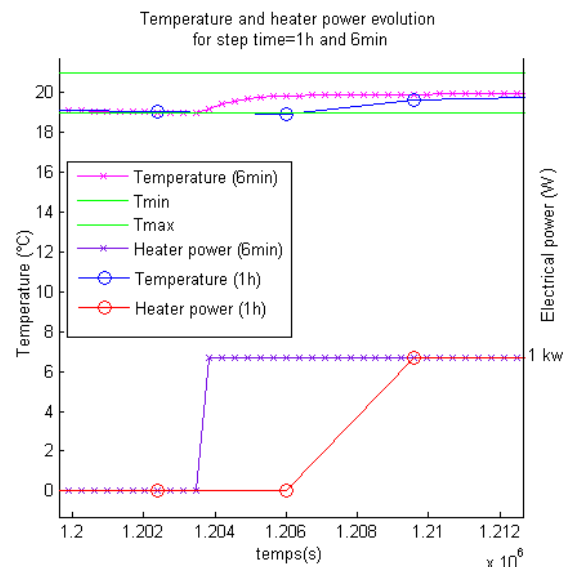
Fig. 1. Temperature and heater power evolution (step time: 1h and 6 min) in MATLAB
