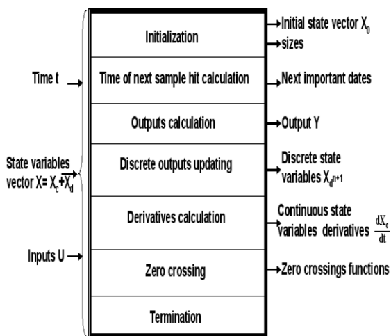
Fig. 3. Hybrid model and solver interactions
