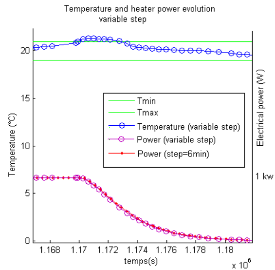
Fig. 6. Variable step time simulation
