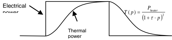
Fig. 4. The heater model
