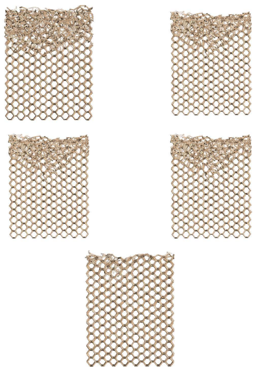
Fig. 6. Evolution of the a -Si/ c -Si [110] interface position during solid phase epitaxy at 1700K. The evolution is reported for respectively 5, 10, 15, 20 and 25 ns illustrating the recrystallisation mechanism where the formation and the dissolution of nanofacets is observed.
