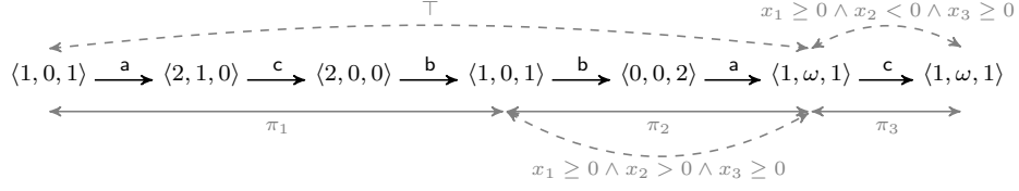
Figure 2: Decomposition of a model for (11).
