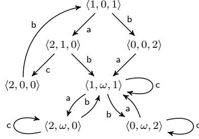
Figure 1: The canonical coverability graph for the VAS \mathcal{S} = \langle \{a, b, c\}, \langle 1, 0, 1 \rangle \rangle with transitions a = \langle 1, 1, -1 \rangle , b = \langle -1, 0, 1 \rangle , and c = \langle 0, -1, 0 \rangle .
