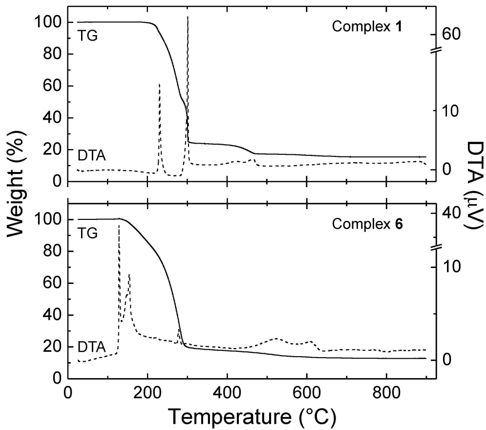
TG/DTA curves for complexes 1 and 6. 103x90mm (600 x 600 DPI)
