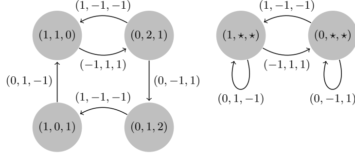
Fig. 1. A subreachability graph G and the subreachability graph \pi_L(G) with L = \{2, 3\} .
