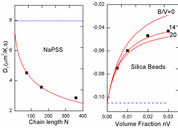
FIG. 2: Comparison with measured data. (a) Variation of D_T with the chain length N of a polyelectrolyte at fixed volume fraction. The data on 2 g/l NaPSS in a 100 mM/l NaCl solution at 30° C are taken from Iacopini et al. [12]. The solid line is calculated from Eq. (13) with the parameters as given in the main text. The dependence on N arises from the gyration radius R . (b) Volume fraction dependence of D_T of a dispersion of 70-nm silica beads in a solution of 30 \mu\text{M} /l sulpho-rhodamine B. The data are from Ghofraniha et al. [14]; the fit curves are obtained from (13) and (16), with different values of the reduced virial coefficient B/V , where V = \frac{4}{3}\pi R^3 is the particle volume.
