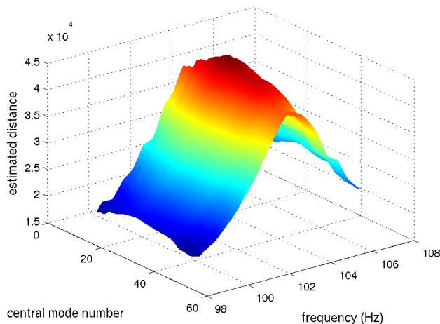
Figure 6: Estimated range distribution slice N = 7 for the Mediterranean data and the striation around 105 Hz
