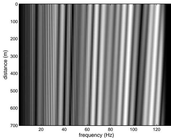
Figure 7: Simulated signal in the Mediterranean environment for a 40 km range
