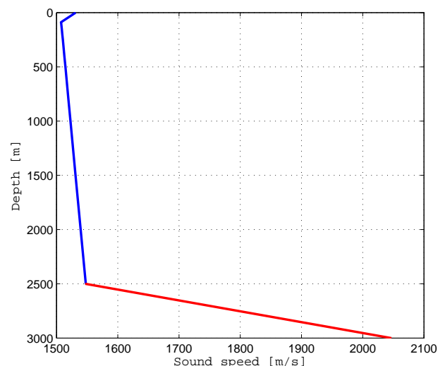
Figure 1: Sound speed profile used for Mediterranean deep water simulation
