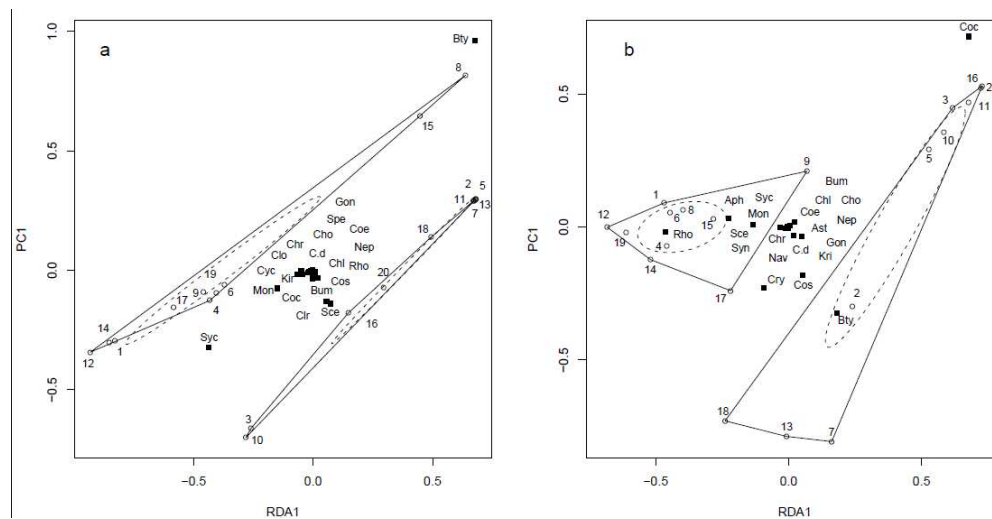
Figure. 3. Redundancy analysis (RDA) biplot for sites (i.e. mesocosms) and species scores for phytoplankton taxa recorded in the mesocosm experiment in April (a) and October (b). In both cases RDA 1 was constrained by treatment and accounted for 24.1% and 24.6% of the variation in the taxonomic composition of the mesocosms in April and October respectively. In the plot the dotted lines denote the 95% confidence ellipses around the centroids for both treatments. In both April and October these ellipses do not overlap indicating that the community composition was significantly different between warmed and ambient treatments. The solid lines enclose all mesocosms that belong to a particular treatment; in both cases heated treatments (1, 4, 6, 8, 9, 12, 14, 15, 17, 19) cluster to the left, while ambient treatments (2, 3, 5, 7, 10, 11, 13, 16, 18, 20) cluster to the right. Genus abbreviations are as follows: Aphanothece (Aph), Asterococcus (Ast), Botryococcus (Bty), Bumilleriopsis (Bum), C.dinobryonis (C.d), Chlorella (Chl), Chlorococcum (Coc), Chroococcus (Chr), Chroomonas (Cho), Coenococcus (Coe), Cosmarium (Cos), Cryptomonas (Cry), Goniochloris (Gon), Kirchneriella (Kri), Monoraphidium (Mon), Navicula (Nav), Nephrocystium (Nep), Rhodomonas (Rho), Scenedesmus (Sce), Synechococcus (Syn), Synechocystis (Syc), Spermatozopsis (Spe).
