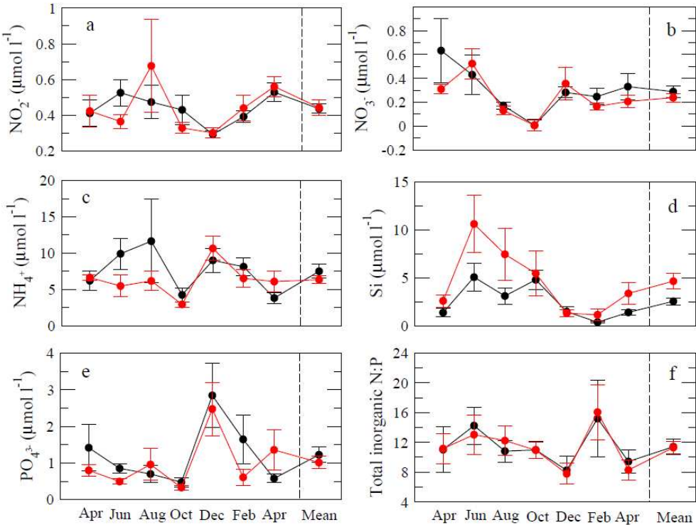
Figure S3. Seasonality of inorganic nutrients in the warmed (red lines) and ambient (black lines) mesocosms. (a) Nitrite, (b) Nitrate, (c) Ammonium, (d) Silicate, (e) Phosphate, (f) the stoichiometry of the inorganic nutrient pool, N:P. Water samples for measuring dissolved inorganic nutrient concentrations were collected from mid depth in the mesocosm at 9am on each sampling occasion. Samples were filtered (Whatmann GF/F) and stored frozen ( -20^{\circ}\text{C} ) for subsequent determination of \text{NO}_3^- , \text{NO}_2^- , \text{NH}_4^+ , \text{PO}_4^{3-} and dissolved silica (Si) using a segmented flow auto-analyser (Skalar, San++, Breda, Netherlands), according to (Kirkwood 1996). Inorganic nutrients ( \text{NO}_3^- , \text{NO}_2^- , \text{NH}_4^+ , \text{PO}_4^{3-} & Si) exhibited strong seasonal trends. For example, \text{NO}_3^- concentrations peaked in spring and declined progressively throughout the summer, when rates of primary production were maximal (Yvon-Durocher et al. 2010), and were depleted to \approx 0.005 \mu\text{mol l}^{-1} by October, before regeneration in the winter. Concentrations of \text{NO}_3^- , \text{NO}_2^- , \text{NH}_4^+ and \text{PO}_4^{3-} showed identical seasonal patterns in the warmed and ambient
