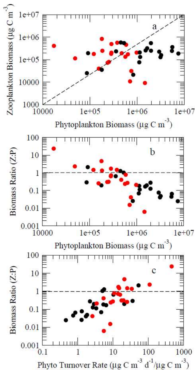
Figure. 6. (a) Relationship between zooplankton and phytoplankton biomass. (b) Relationship between the ratio of zooplankton to phytoplankton biomass (Z:P) and total phytoplankton biomass. (c) The relationship between Z:P and the turnover rate of the phytoplankton communities. Each data point corresponds to either the total zooplankton or phytoplankton biomass or the Z:P in either a heated (red circles) or ambient mesocosm (black circles). 180x328mm (72 x 72 DPI)
