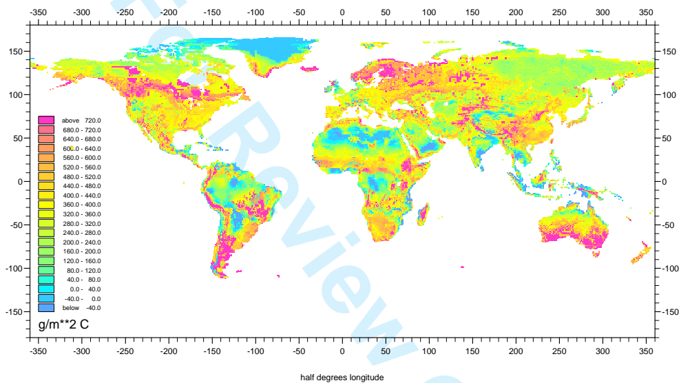
Figure 9: Change of the carbon storage in soil from 1860 to 2002 AD [g·m -2 ] as calculated with NCIM using the configuration of experiment 4 (cn_full) (see table 7).
