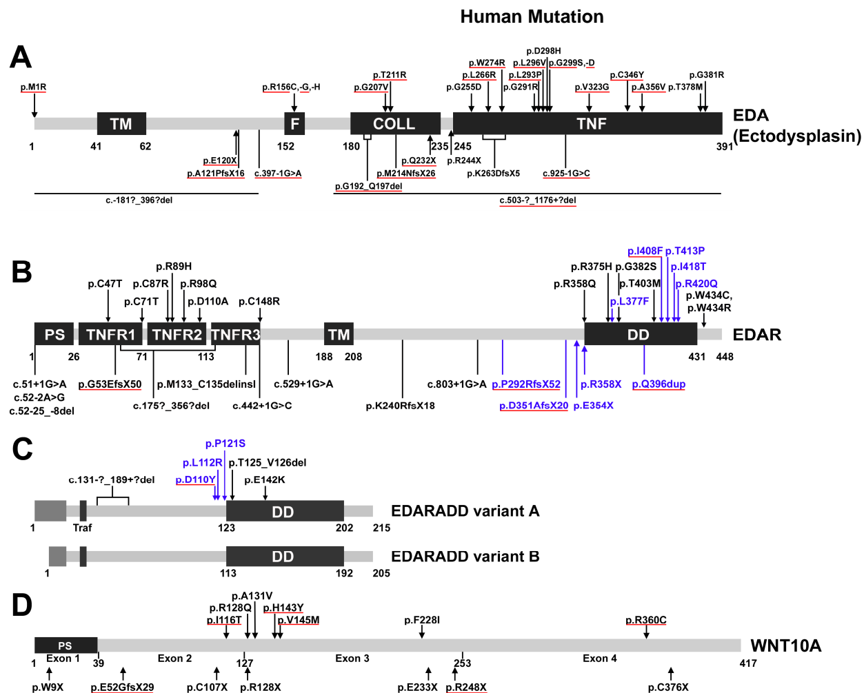
Supp. Figure S1: Distribution of previously known and newly identified mutations regarding to functional domains of EDA1 (A), EDAR (B), EDARADD (C) and WNT10A proteins (D). Missense mutations are indicated above the schematic representation of each protein, whereas nonsense, splice and truncating mutations are positioned underneath. Mutations with a dominant mode of inheritance in EDAR and EDARADD figure in blue; newly identified mutations are underlined in red. Ectodysplasin is mainly mutated in its furin cleavage site, its collagenous and its TNF domains. Mutations in EDAR are located either in the N-terminal ligand binding domain, or in the C-terminal Death Domain (DD). Interestingly, all dominant EDAR mutations are located in its C-terminal region. All EDARADD missense mutations are located in or very close to its Death Domain. TM: transmembrane domain; F: furin cleavage site; COLL: collagen domain; TNF: TNF-like domain; PS: peptide signal; TNFR1 to -3: TNF Receptor like domain; DD: Death domain. Reference sequences used to annotate all mutations are: NP_001390.1 (EDA1), NP_071731.1 (EDAR), NP_080738.3 (EDARADD), NP_079492.2 (WNT10A).
