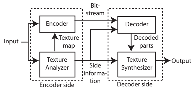
Figure 1: Framework overview.
