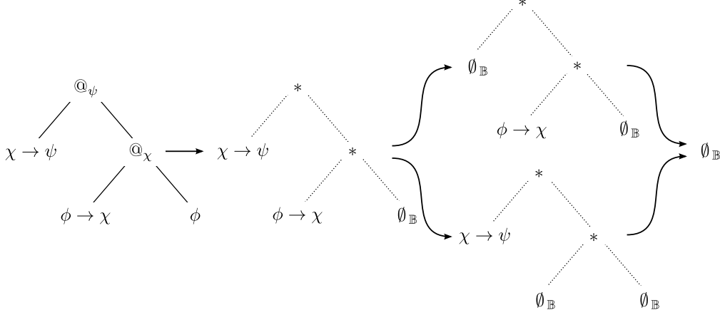
Fig. 5. Full reductions of @_\psi(\chi \rightarrow \psi, @_\chi(\phi \rightarrow \chi, \phi)) to \emptyset_{\mathbb{B}} .
