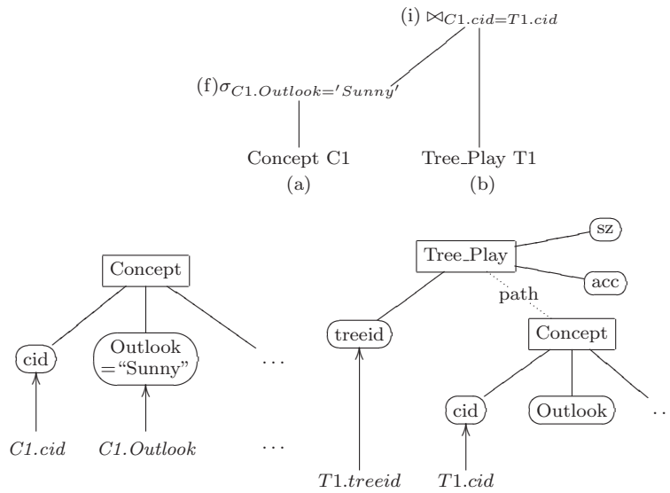
Fig. 21 Annotation for R_f \times R_b (bottom) and node (i) as seen in the example algebra tree (top).
