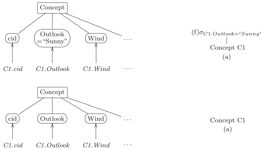
Fig. 20 Annotation for node (f) (top left), its corresponding sub-query (top right), and the annotation for its child node, (a) (bottom).
